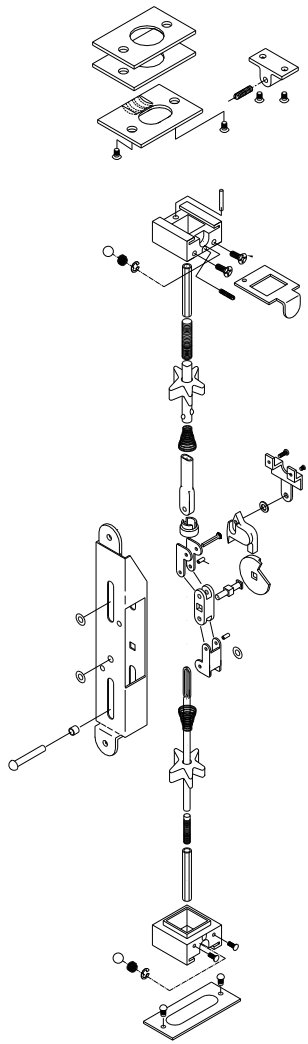
1085/2086 ROD AND CASE ASSY 30-915
